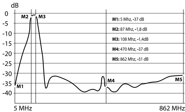
Coupling attenuation IN→R
